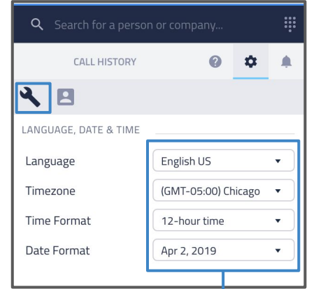
Settings > General
