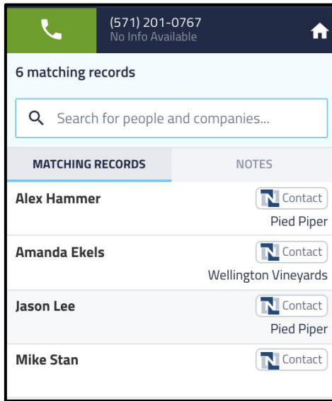
Multiple Match
