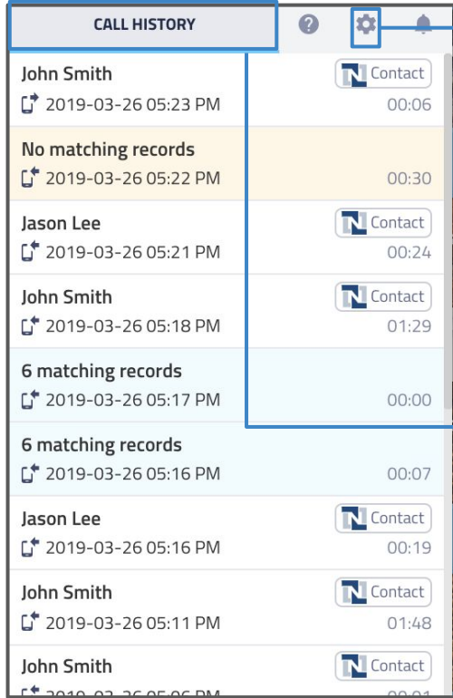
Home Page
