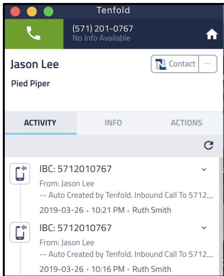
Single Match
