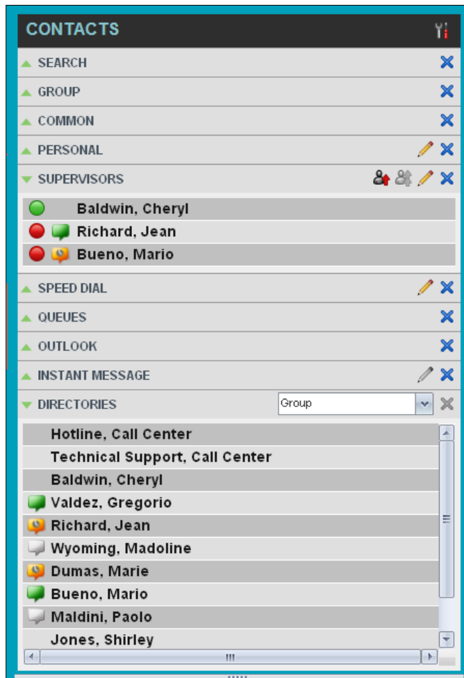
Figure 20 Contacts Pane
