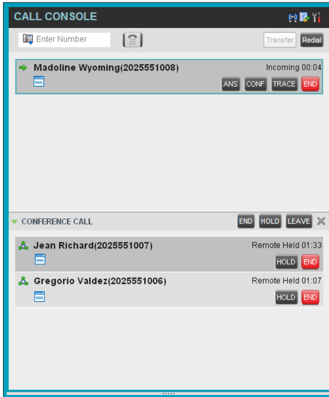
Figure 15 Call Console
