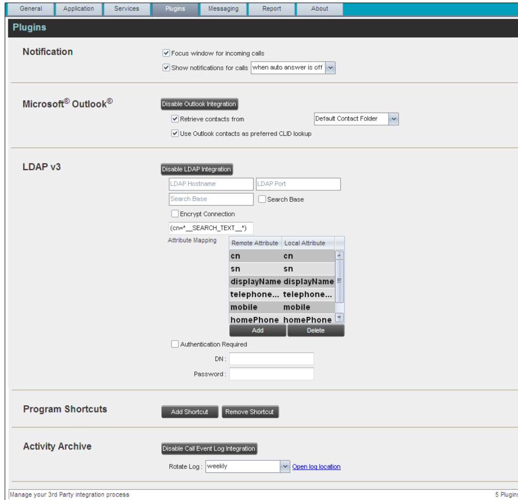
Figure 107 Settings – Plugins
