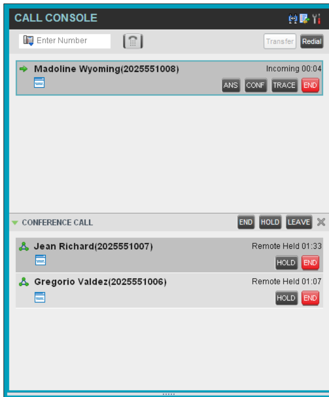
Figure 34 Call Console
